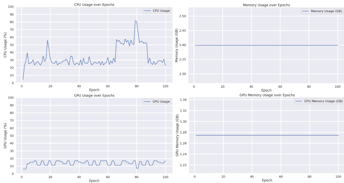
Figure 20: Training GCN with Amazon Computers - GPU Accelerated.
