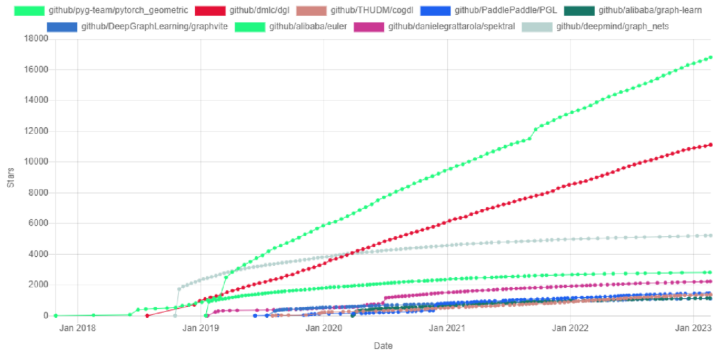
Figure 8: GNN Engines GitHub Stars.
