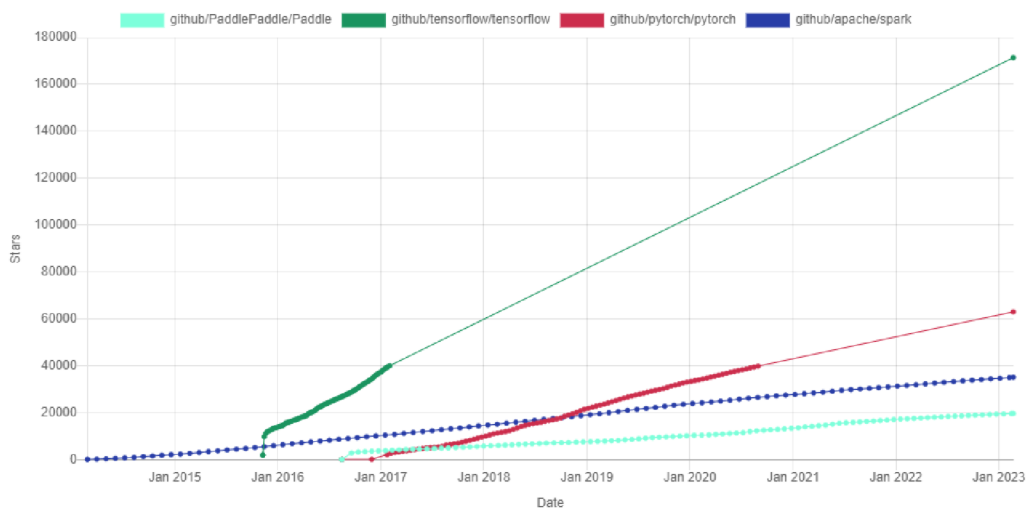
Figure 6: General Purpose Analytical Engines GitHub Stars.
