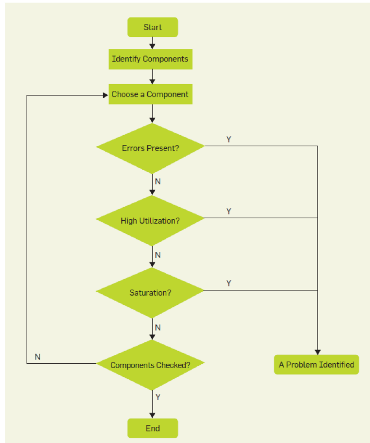
Figure 9: The USE Method.
