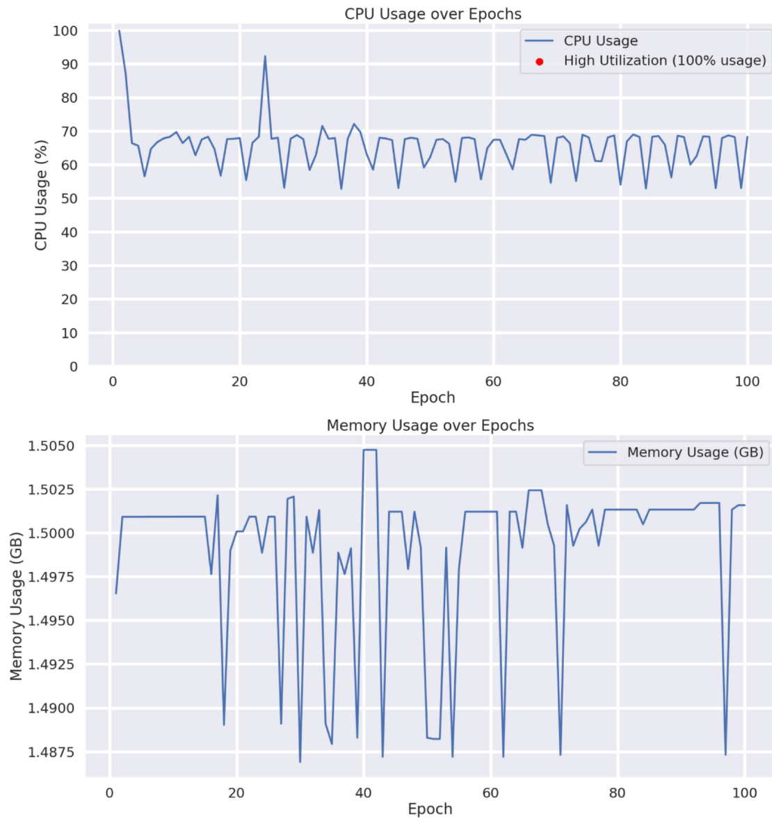
Figure 29: Training GraphSAGE with CoAuthors CS - CPU only.
