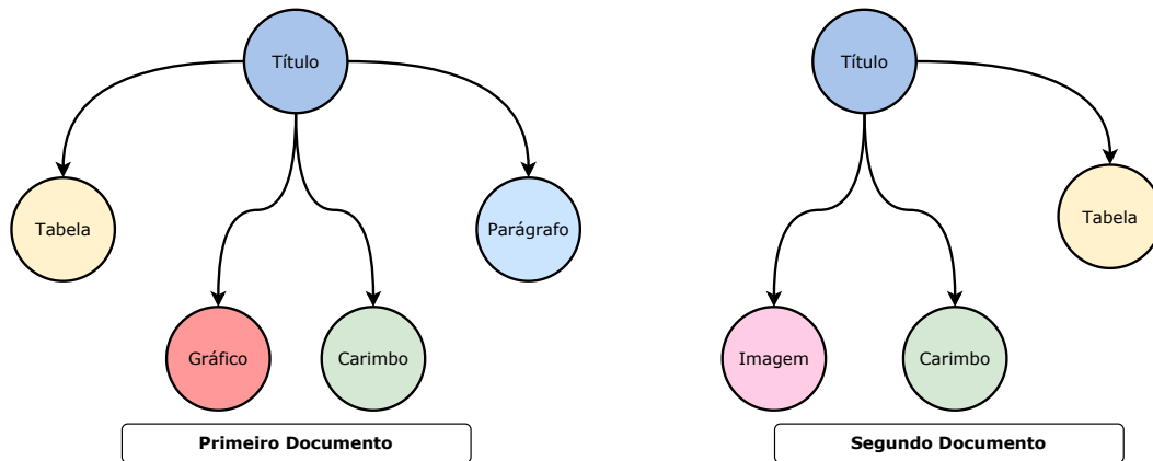
Figure 2: Representing documents in a graph model.
