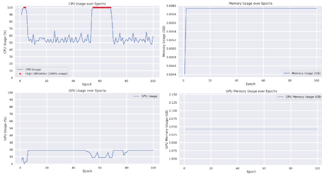
Figure 24: Training GCN with CoAuthors CS - GPU Accelerated.
