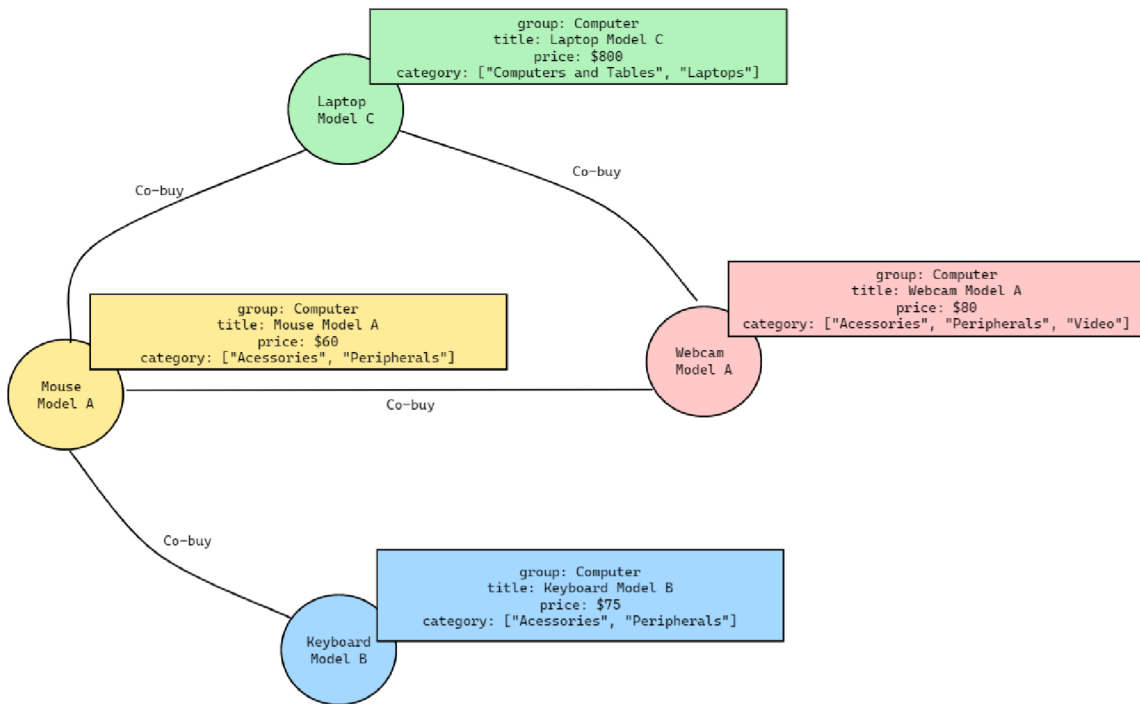
Figure 11: Amazon Computers (or AmazonCoBuy) Representation.
