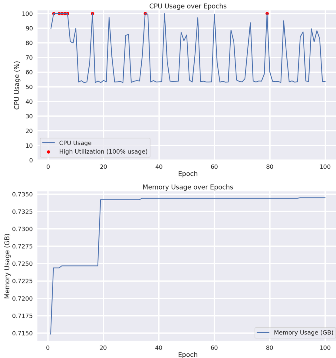
Figure 25: Training GraphSAGE with Amazon Computers (CPU only) resources.
