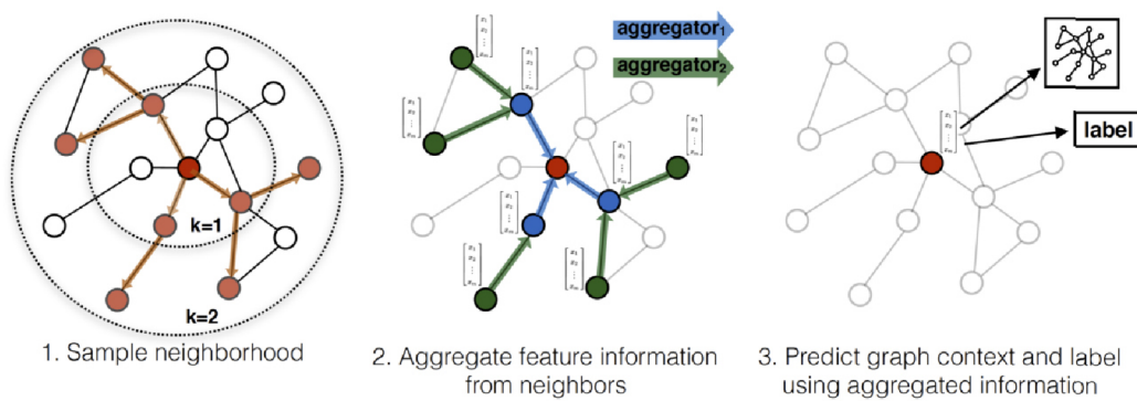
Figure 3: Node Classification with GraphSAGE.
