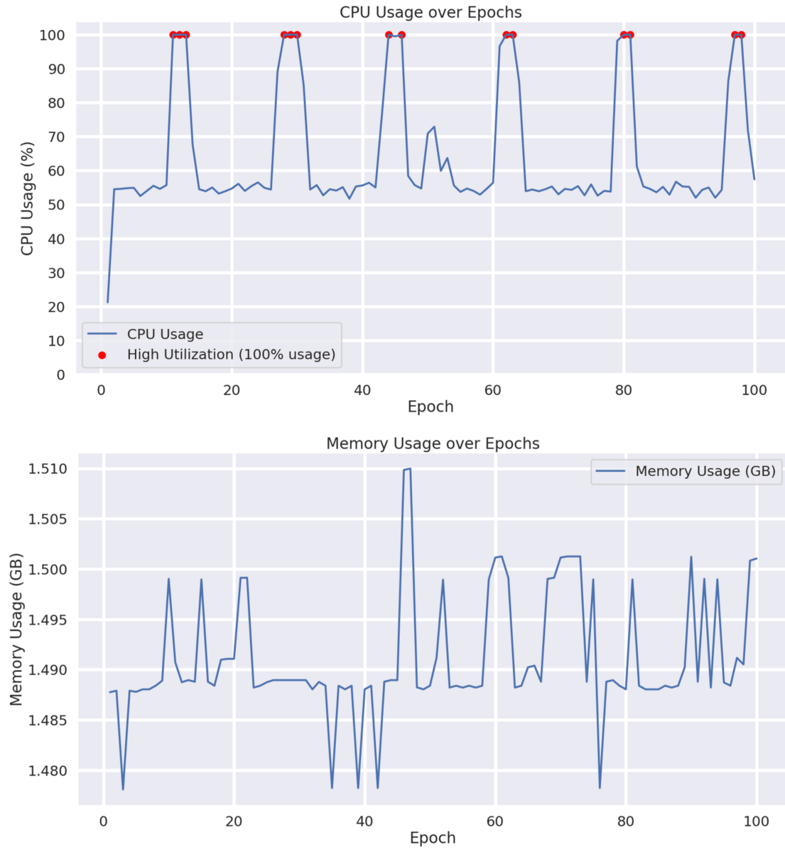
Figure 23: Training GCN with CoAuthors CS - CPU only.
