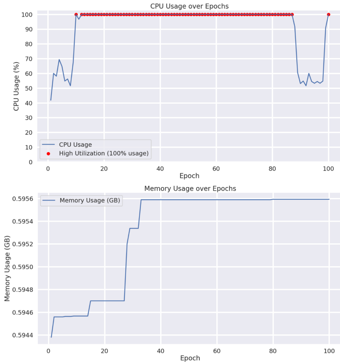
Figure 27: Training GraphSAGE with CiteSeer - CPU only.
