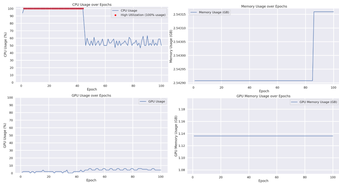
Figure 28: Training GraphSAGE with CiteSeer - GPU Accelerated.
