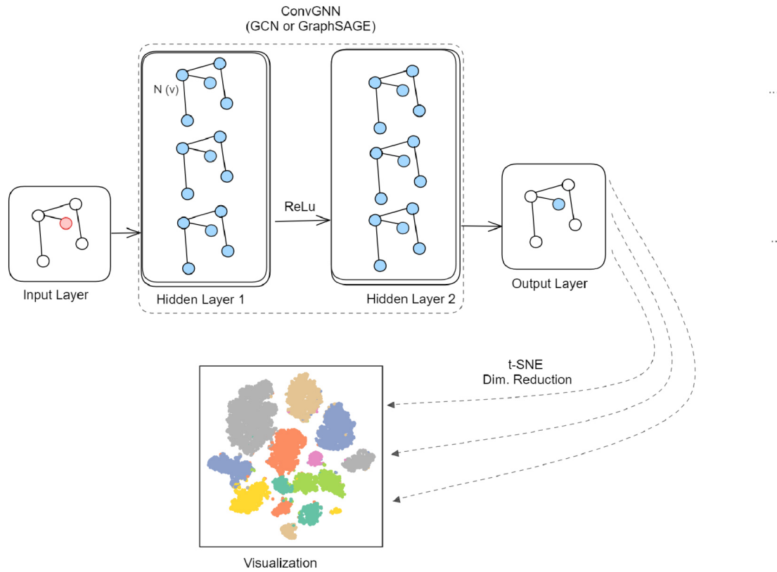
Figure 10: Representational Diagram of the used models (GCN and GraphSage).
