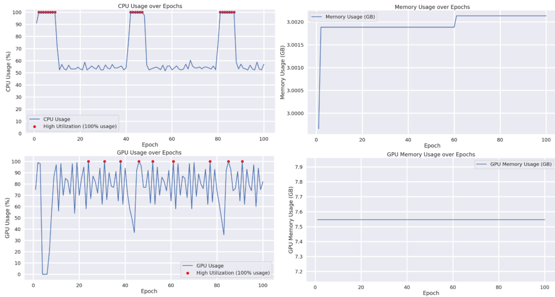
Figure 30: Training GraphSAGE with CoAuthors CS - GPU Accelerated.
