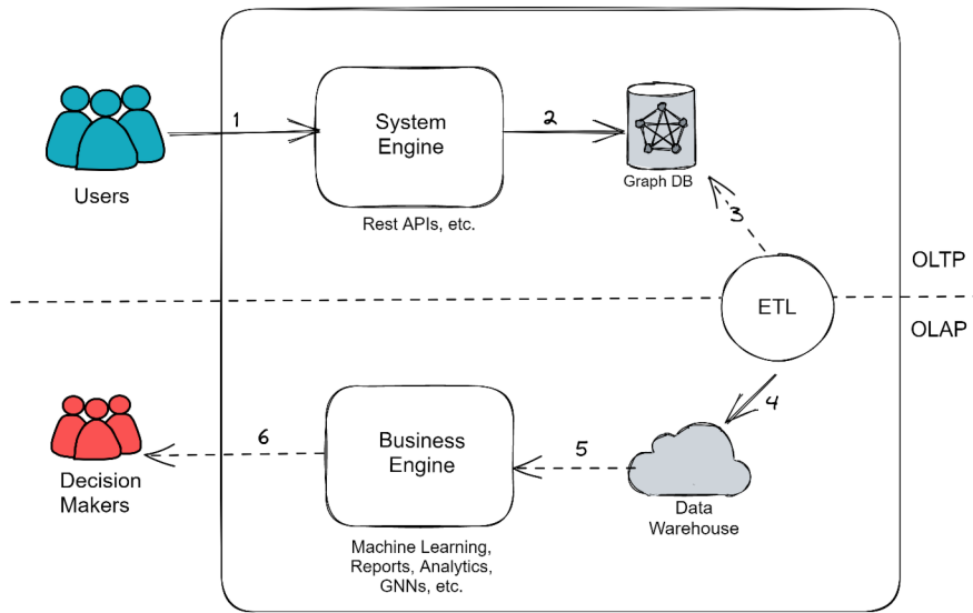
Figure 1: Pipeline for a graph application with both OLTP and OLAP.
