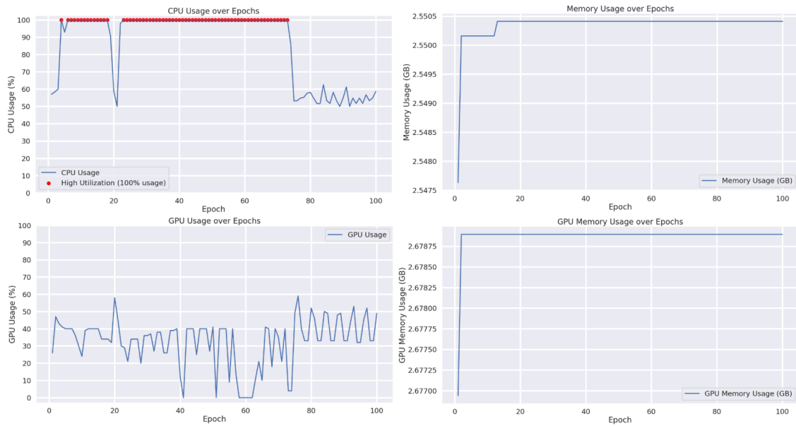
Figure 26: Training GraphSAGE with Amazon Computers - GPU Accelerated.
