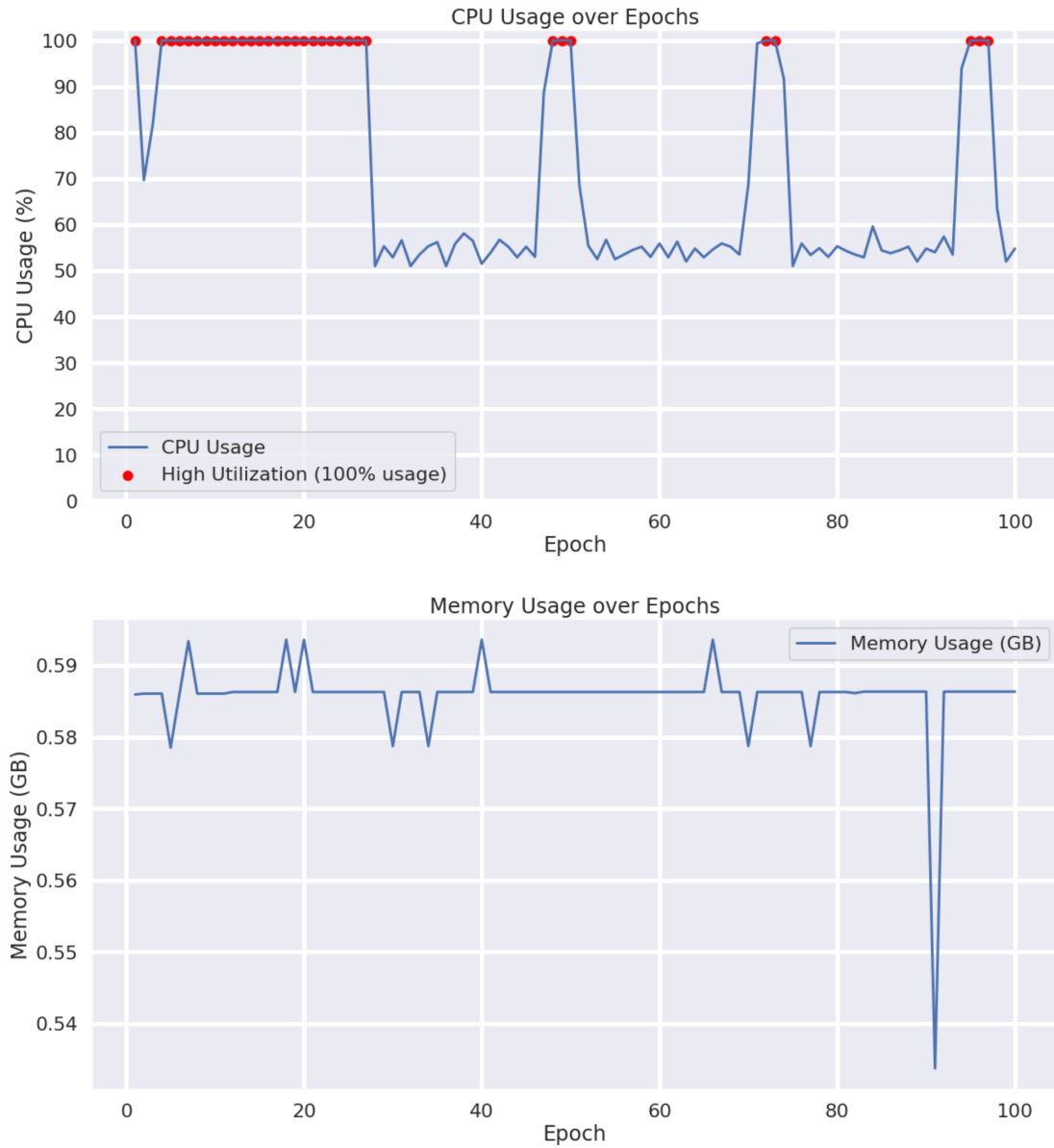
Figure 19: Training GCN with Amazon Computers - CPU only.
