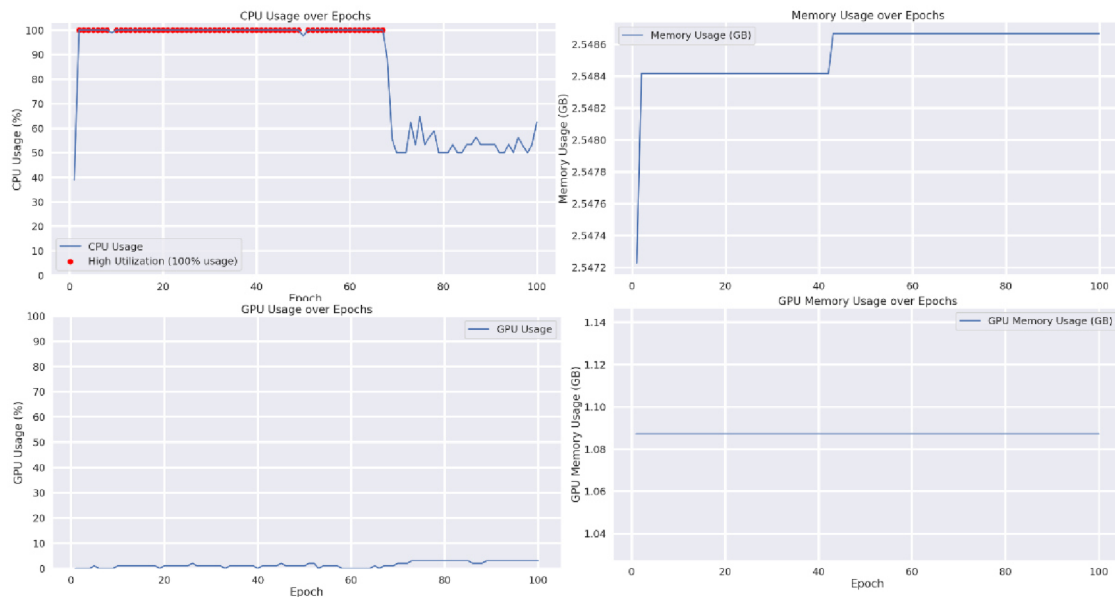
Figure 22: Training GCN with CiteSeer - GPU Accelerated.
